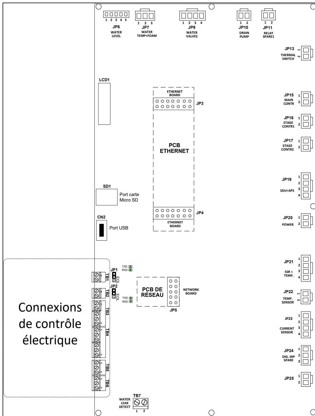
Illustration 38 - Circuit imprimé
